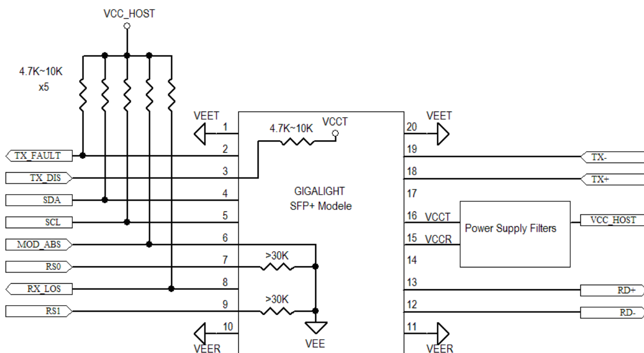
Figure4. Host-Module Interface
